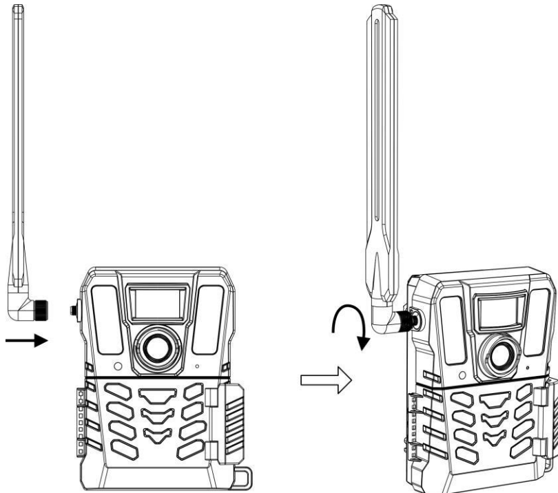
Figure 2-4 Install Antenna
