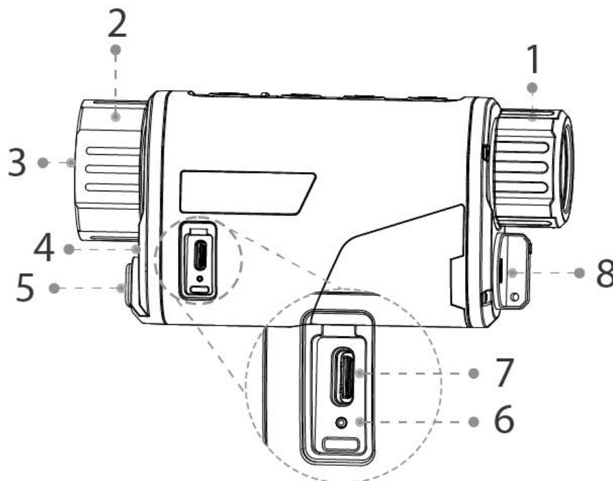
Figure 2-3 Port description
