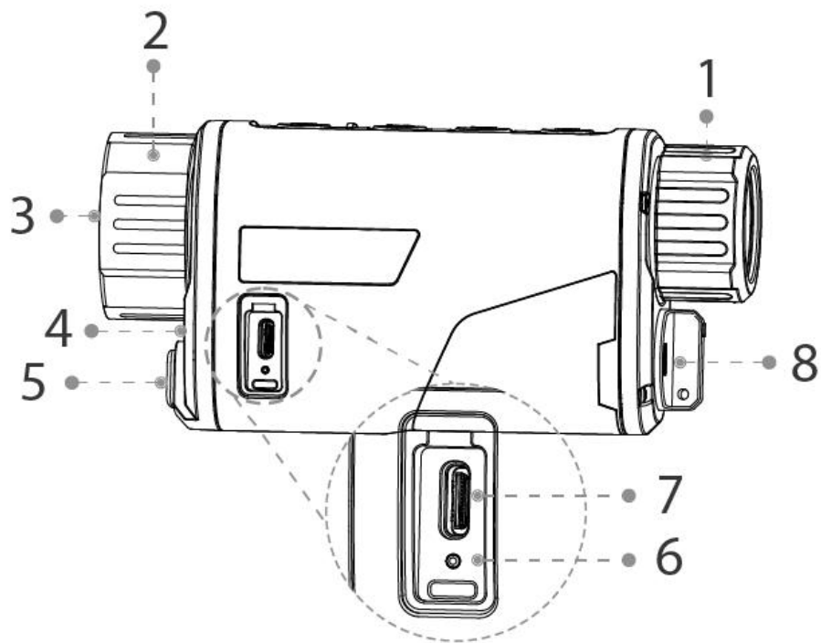
Figure 2-3 Port description
