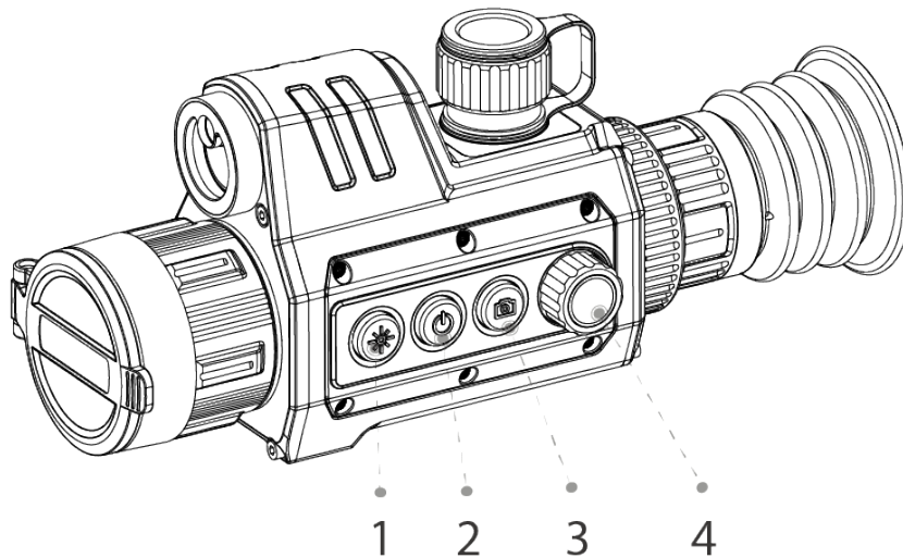
Figure 2-2 Button description
